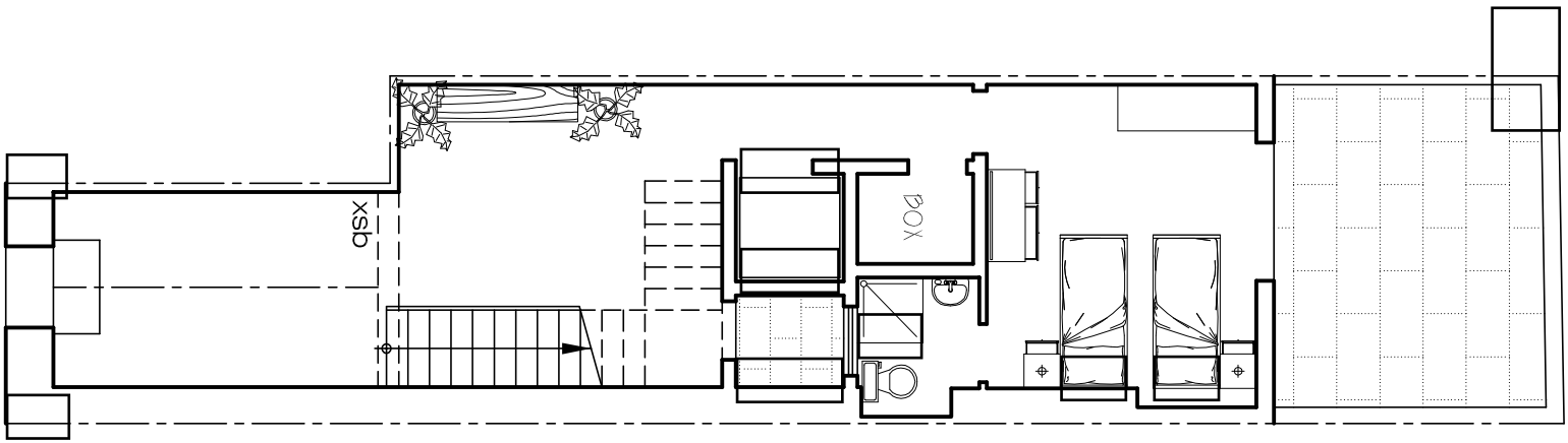
GROUND FLOOR PLAN 1:100
