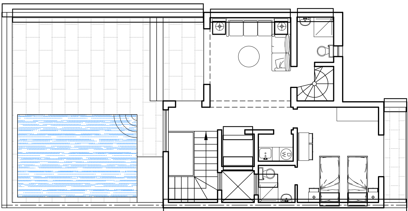
ROOF PLAN 1:100
